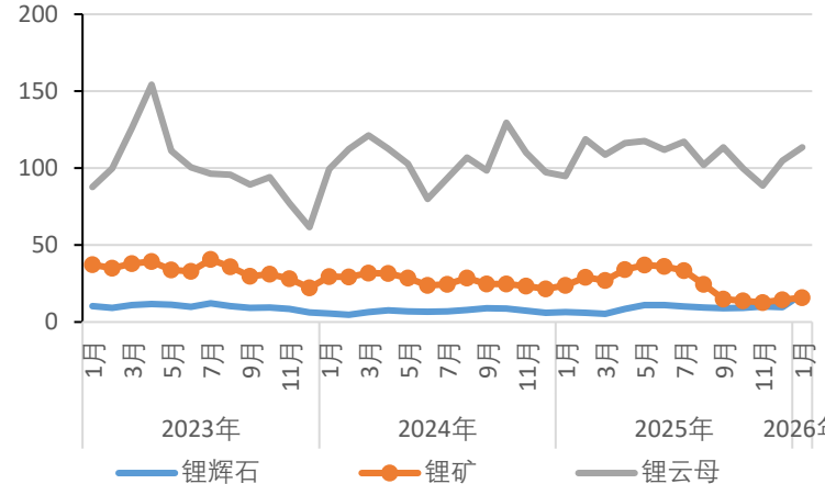
锂矿自给率
