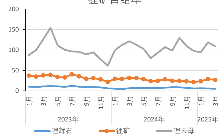
锂矿自给率
